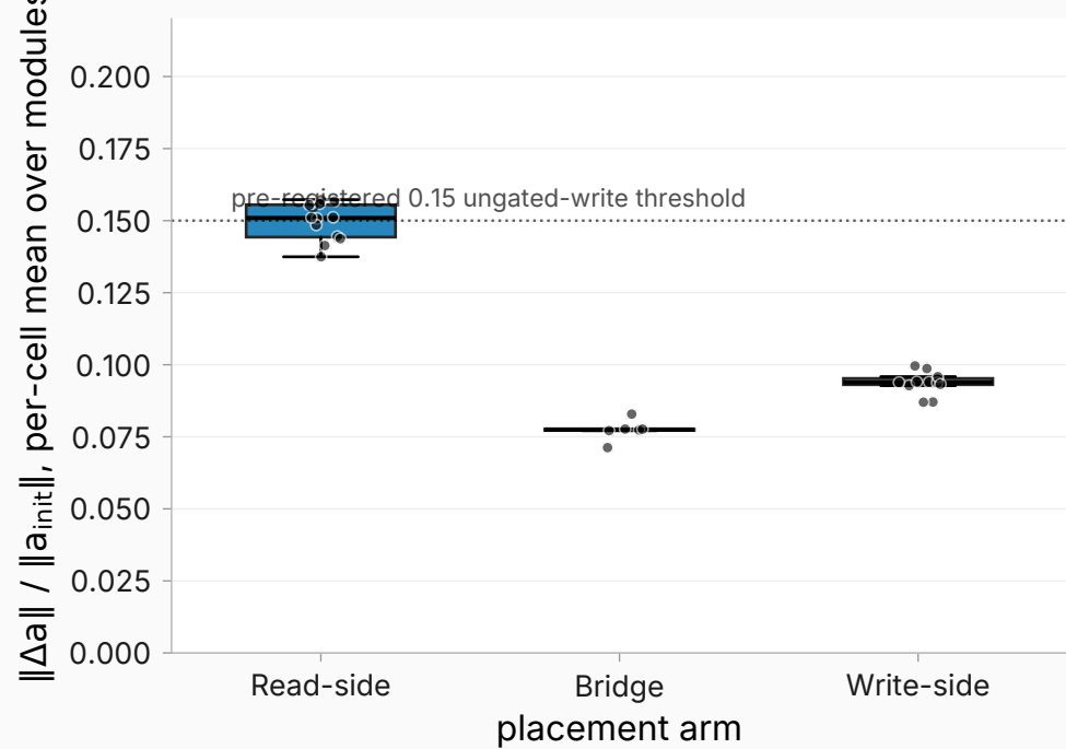
(b) Net A rotation under 16% of its initial norm
