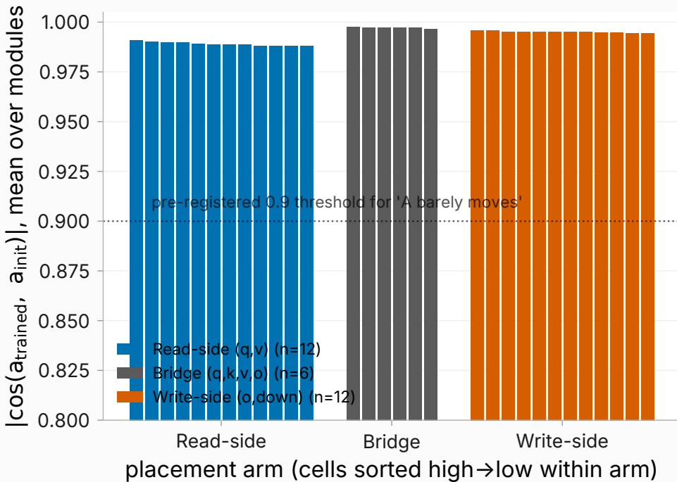
(a) A barely rotates from random init
