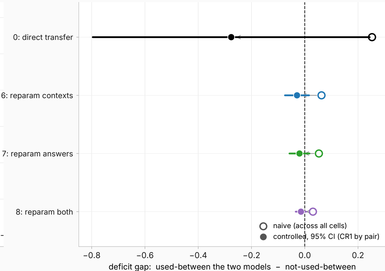
Naive gap → gap with pair and corpus effects removed
