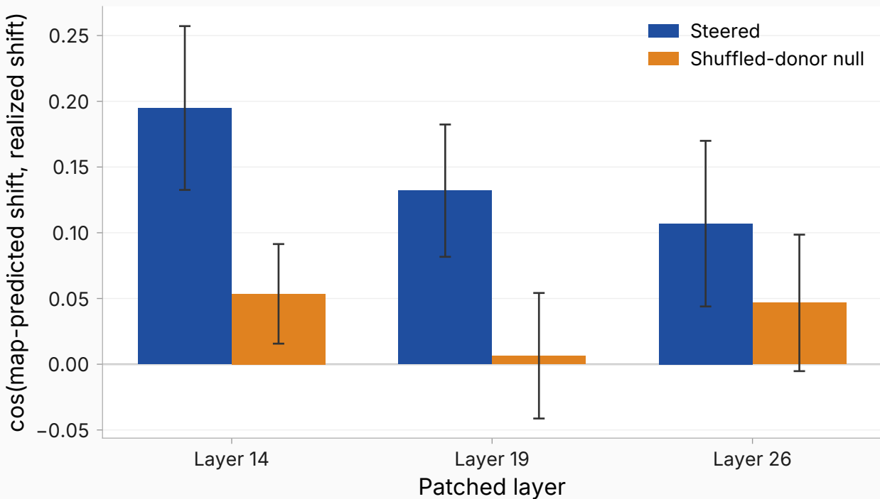
Matched-query full-state patch, context-end
