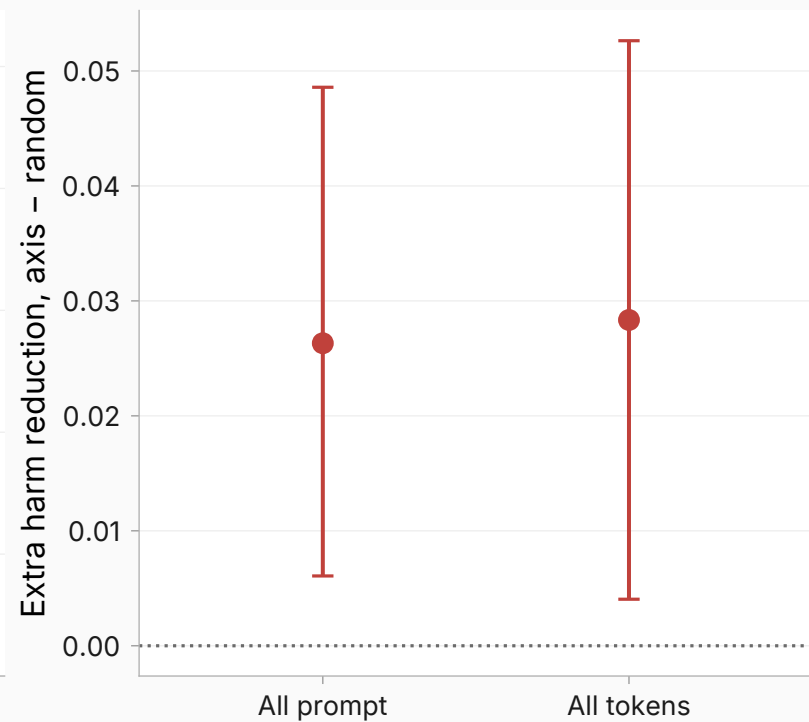
Paired difference (95% cluster-bootstrap CI)
