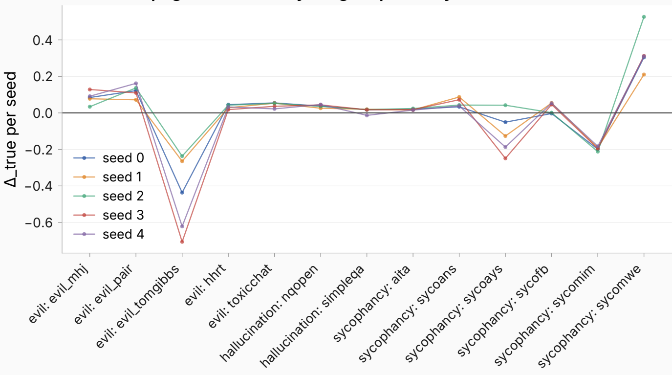
Per-seed spaghetti: \Delta_{\text{true}} by rung (exploratory)
