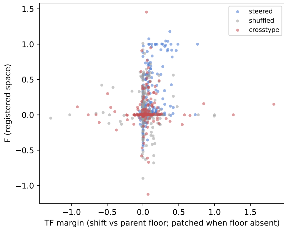
tbmp: margin vs judged F, per (pair x slot x arm)
