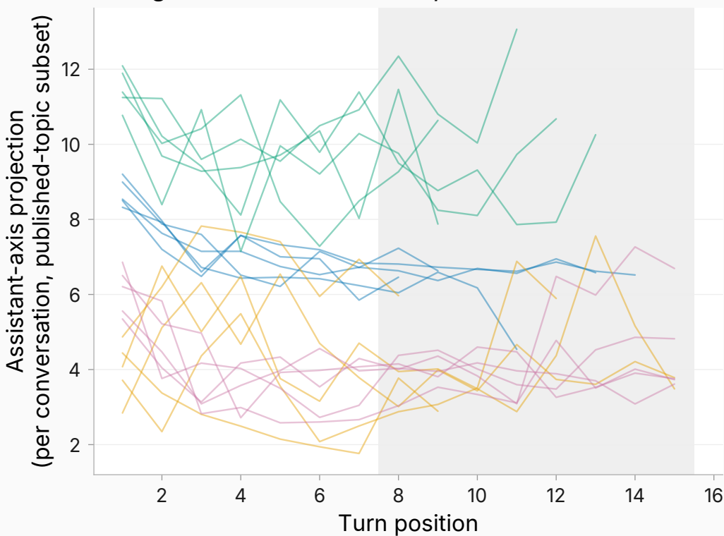
7B leg (Qwen2.5-7B-Instruct, in-house axis)
