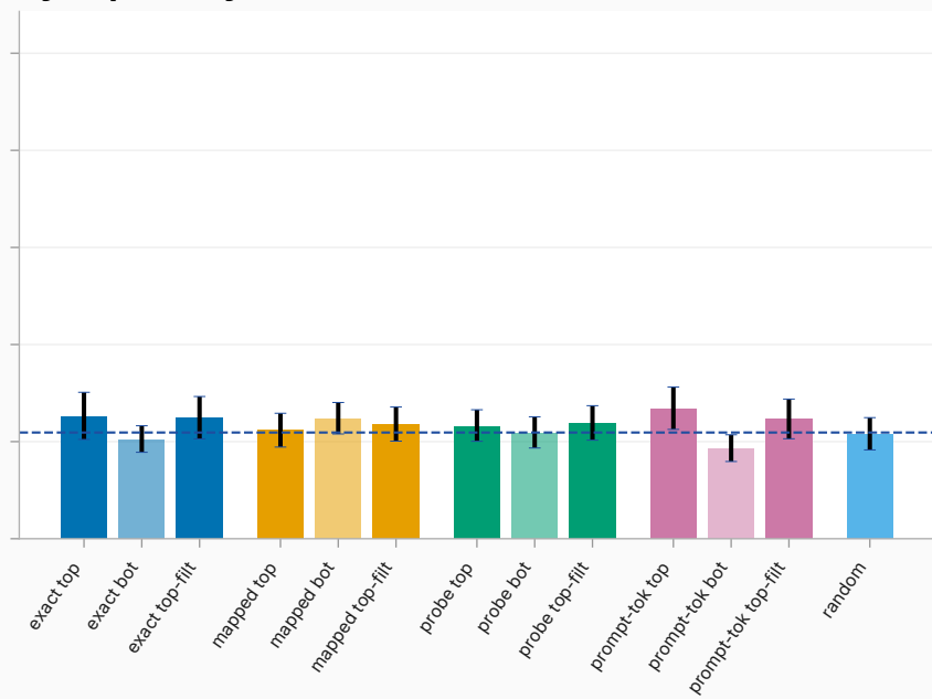
4b selection-finetune trait expression — lmsys (dashed: base model; †: incoherent-flagged cell)
