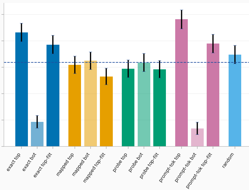
4b selection-finetune trait expression — lmsys (dashed: base model; †: incoherent-flagged cell)
