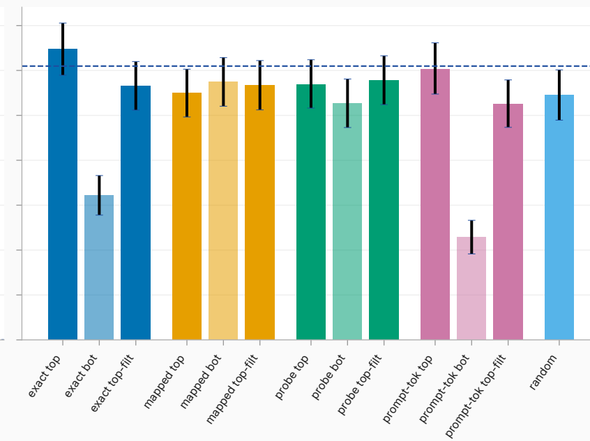
4b selection-finetune trait expression — ultrachat (dashed: base model; †: incoherent-flagged cell)
