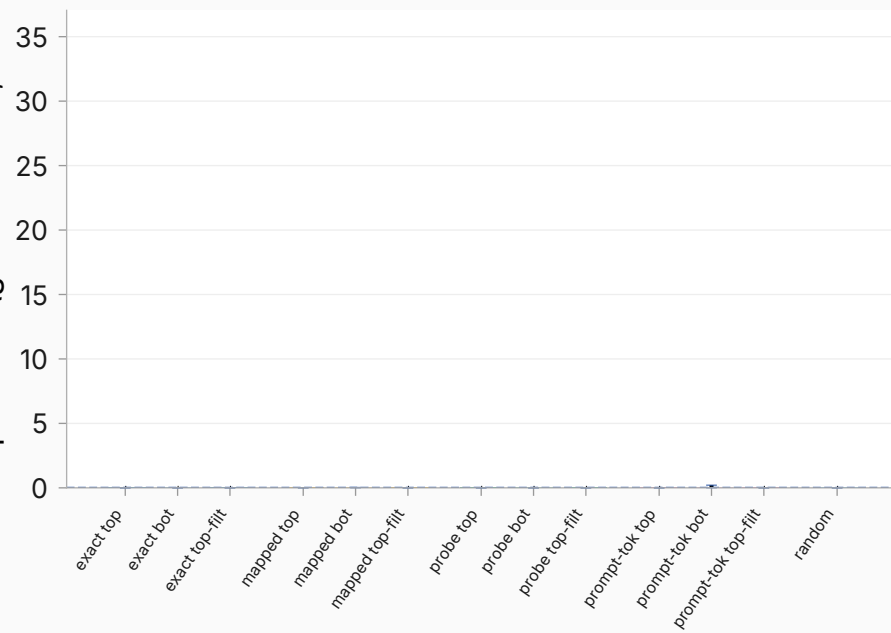
4b selection-finetune trait expression — ultrachat (dashed: base model; †: incoherent-flagged cell)
