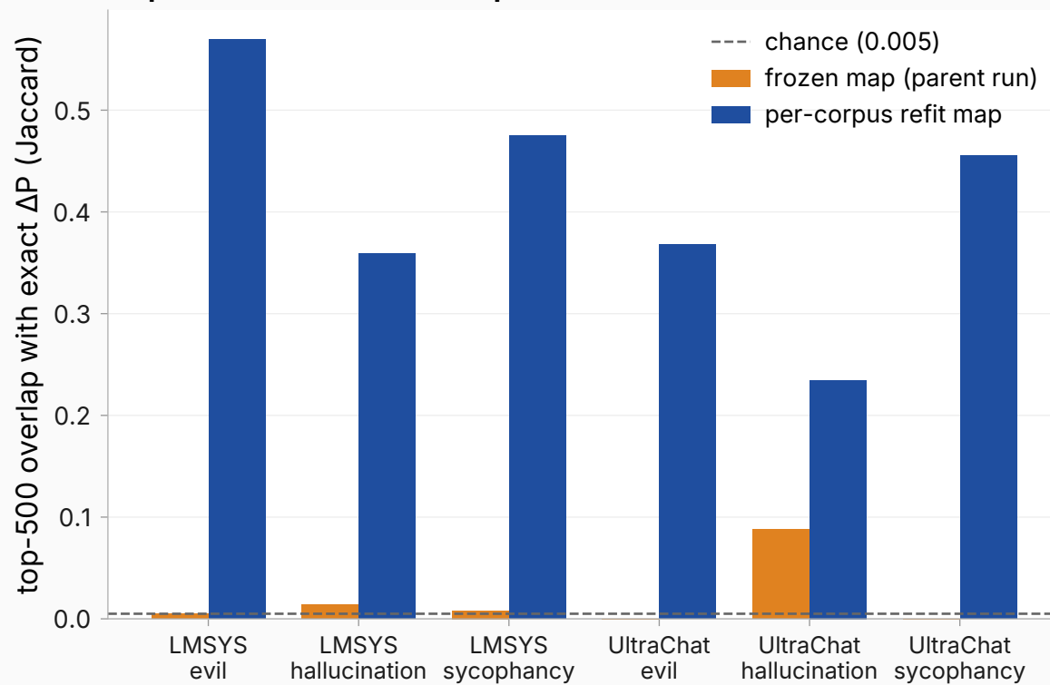
Top-500 selection overlap with exact \Delta P
