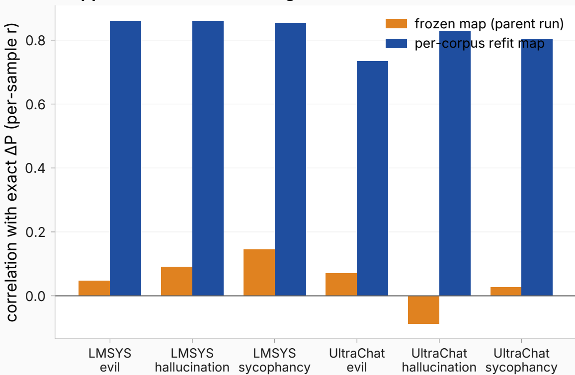
Mapped-score calibration against exact \Delta P
