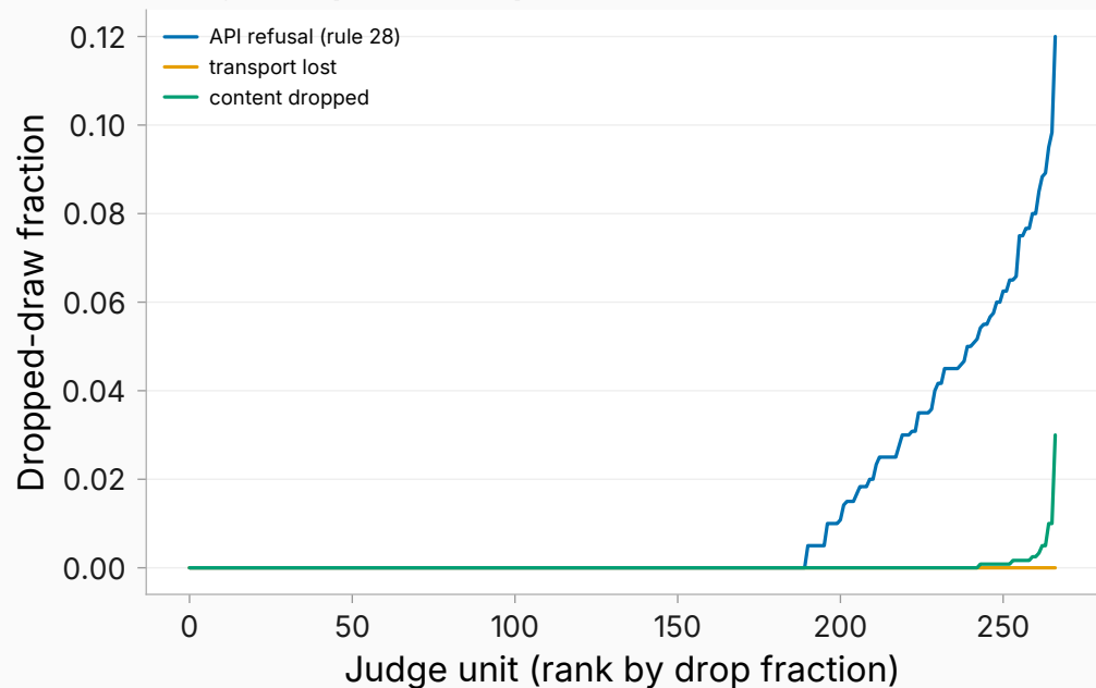
Judge drop classes per unit
