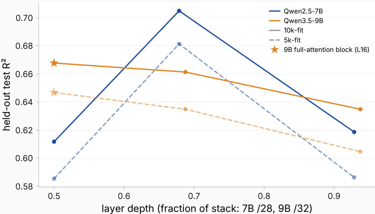
Per-layer map R^2 at depth-matched capture layers
