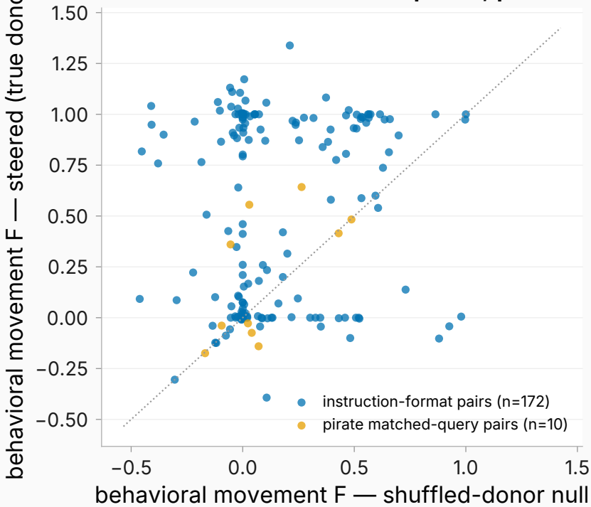
Qwen2.5-7B: three-token prefill, patch-content donors — per pair
