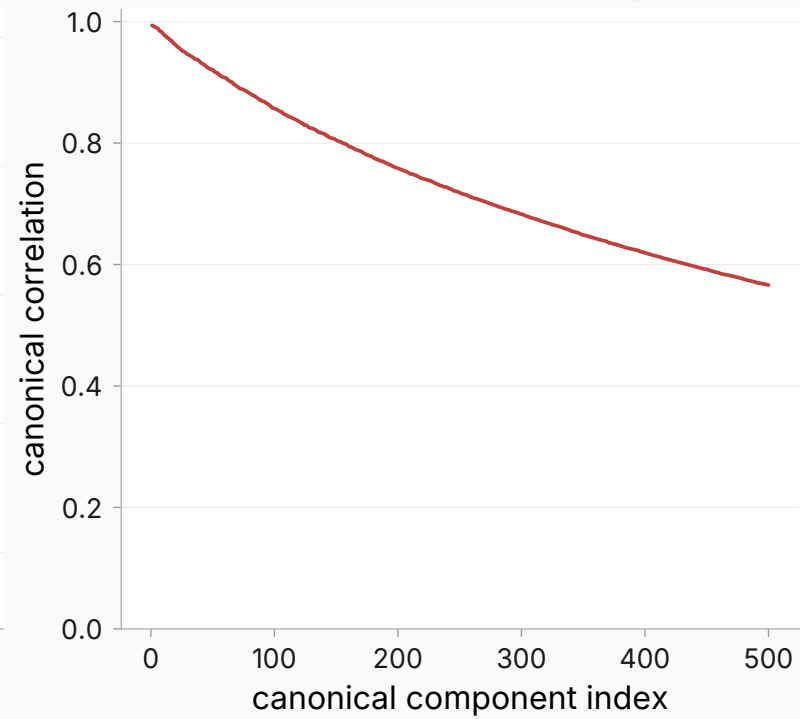
context \leftrightarrow true-answer CCA spectrum
