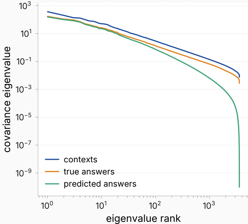
eigenvalue spectrum (log-log)
