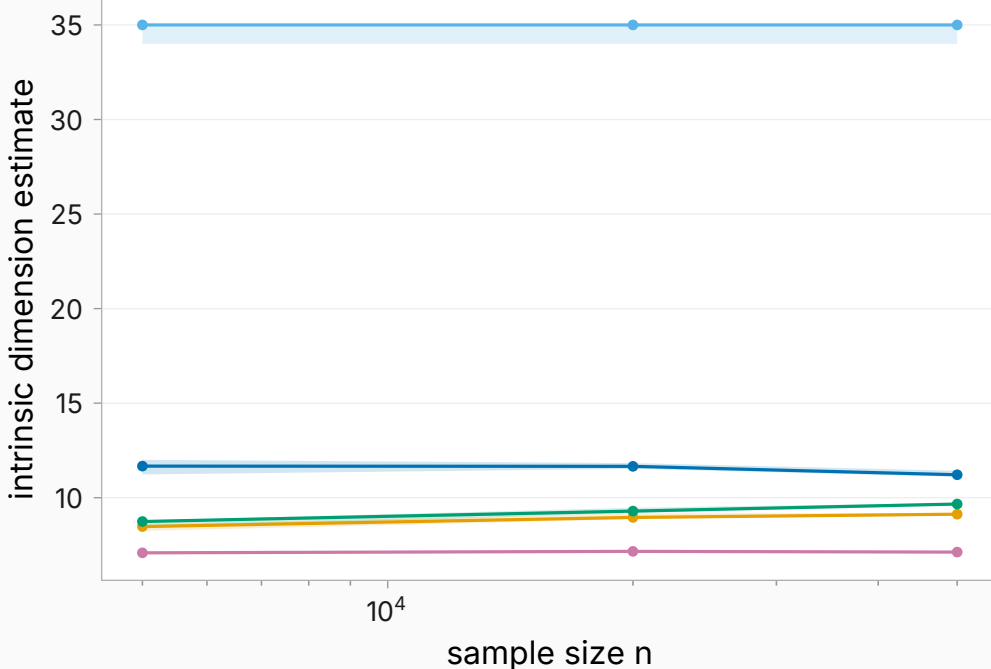
predicted answers (ambient dim 3584)
