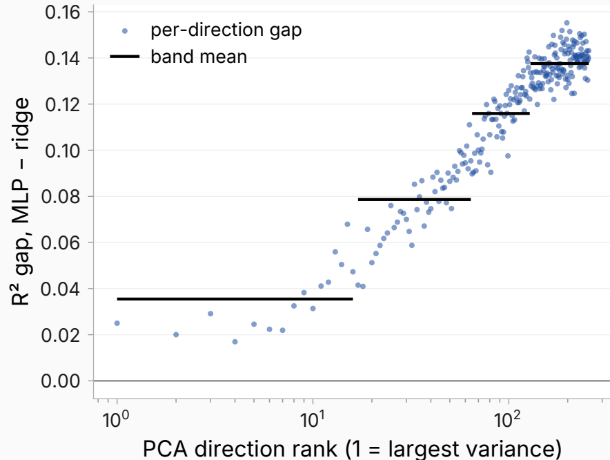
Linear-vs-nonlinear gap per direction
