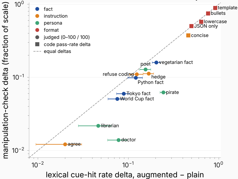
Per-instance delta: lexical screen vs manipulation check
