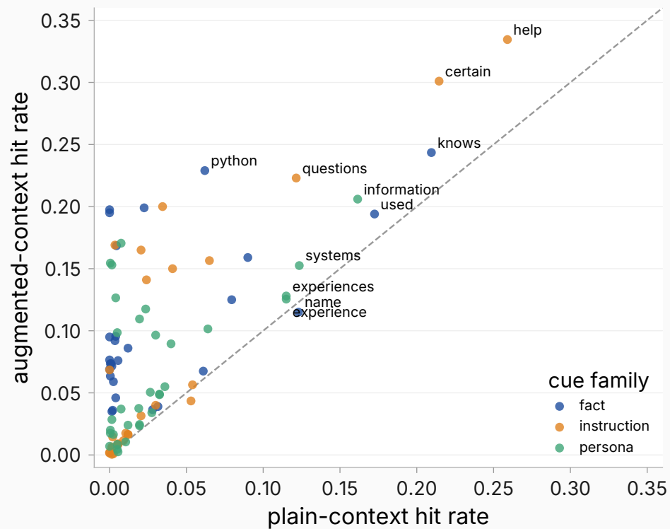
Per-cue hit rates behind the instance deltas
