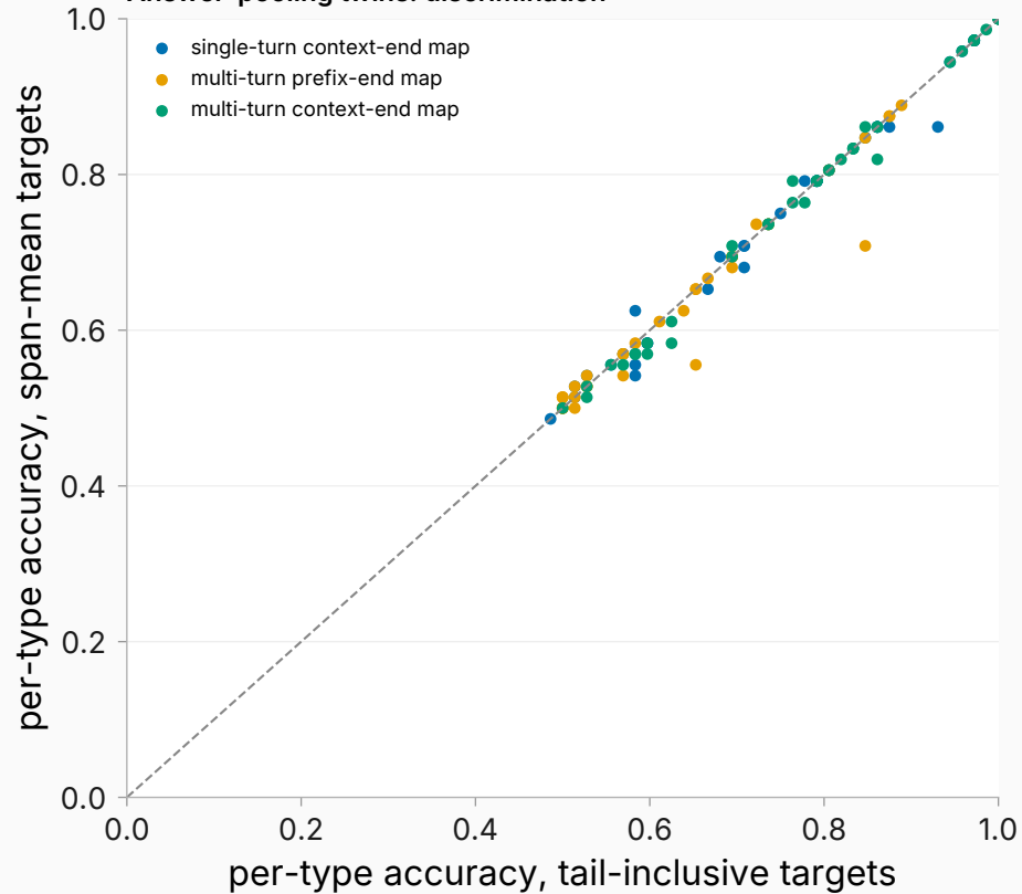
Answer-pooling twins: discrimination
