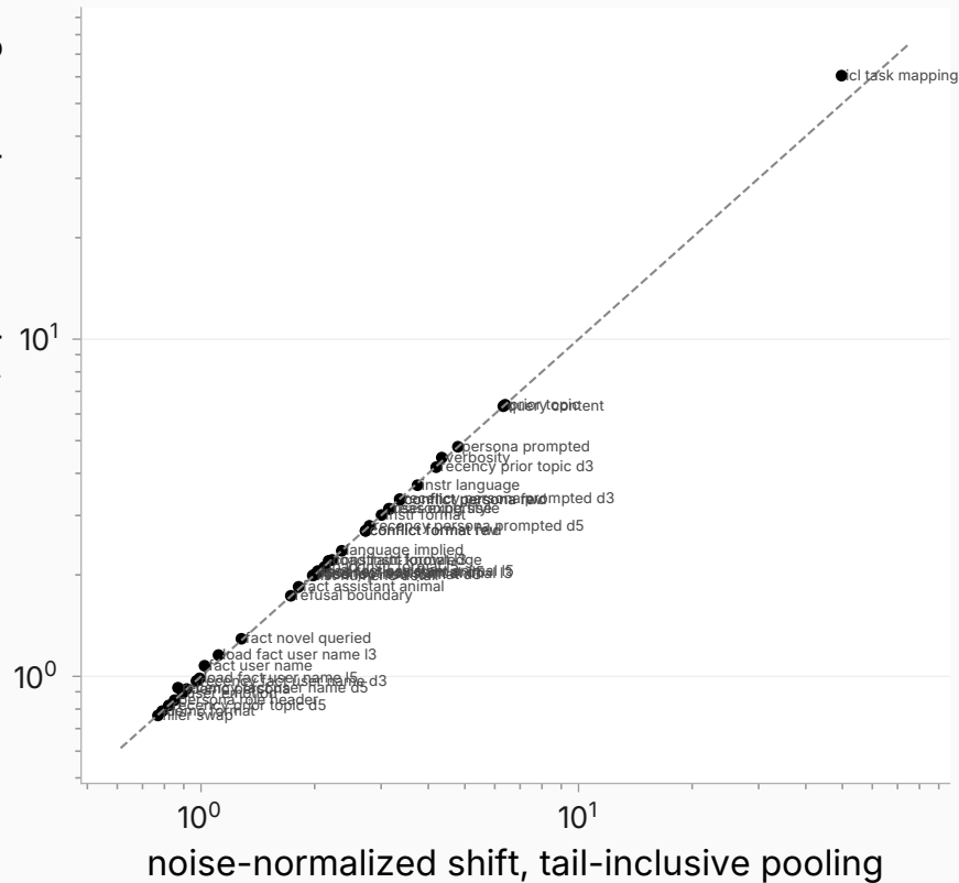
Answer-pooling twins: shift magnitude
