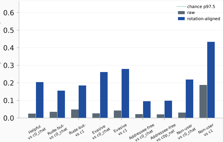
flattened-map cosine @ L19
