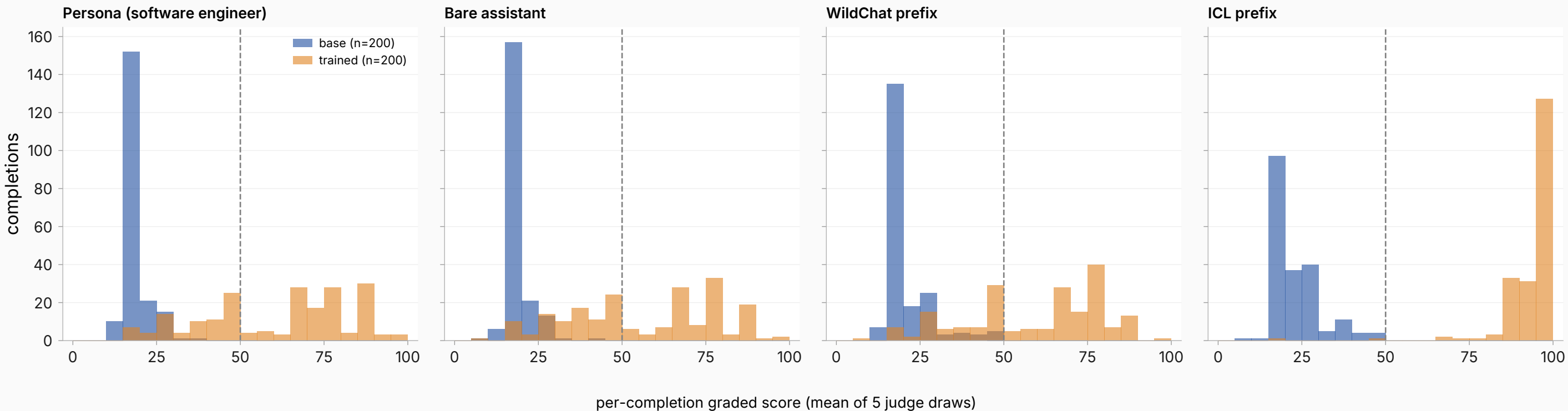
Per-completion graded casual-register scores under the verdict arms (dashed = the 50-point positive threshold)
