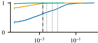
parent token-level SAE on turn averages, layer 20
