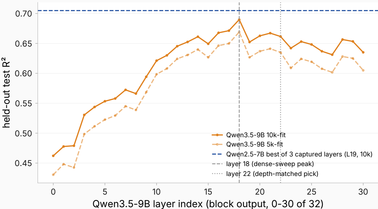
Dense per-layer map R^2 , Qwen3.5-9B
