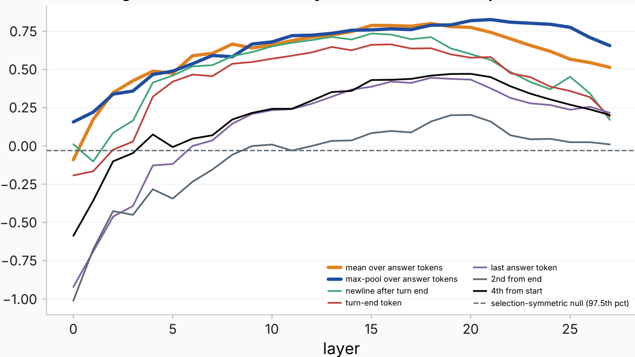
Predicting each answer summary from the context representation
