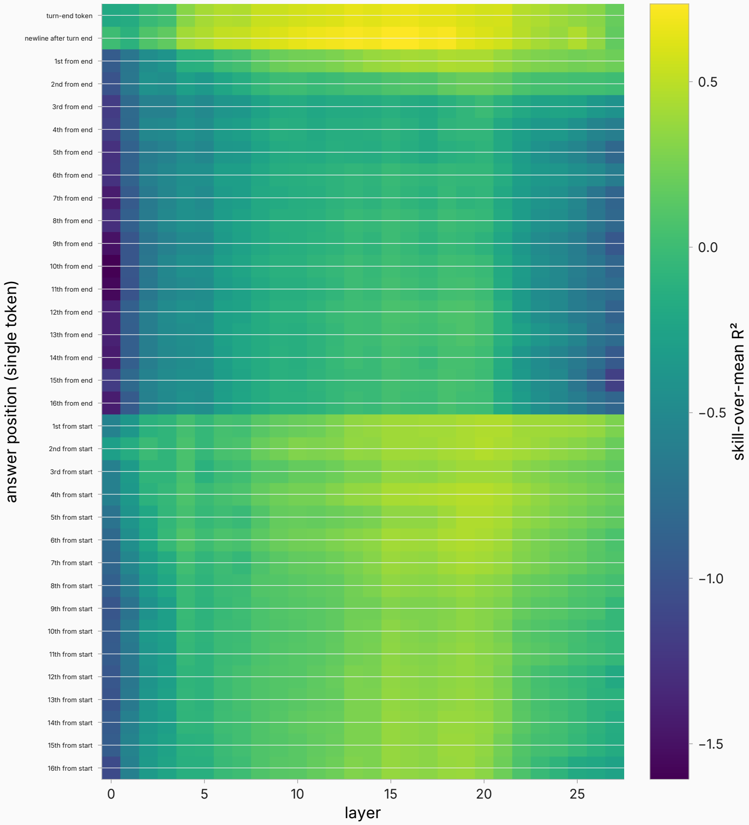
Reconstruction skill per answer position × layer
