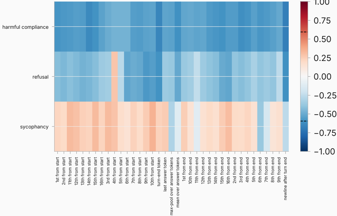
fixed behavior-direction read-out null band (97.5th pct of max): |\rho| \leq 0.595
