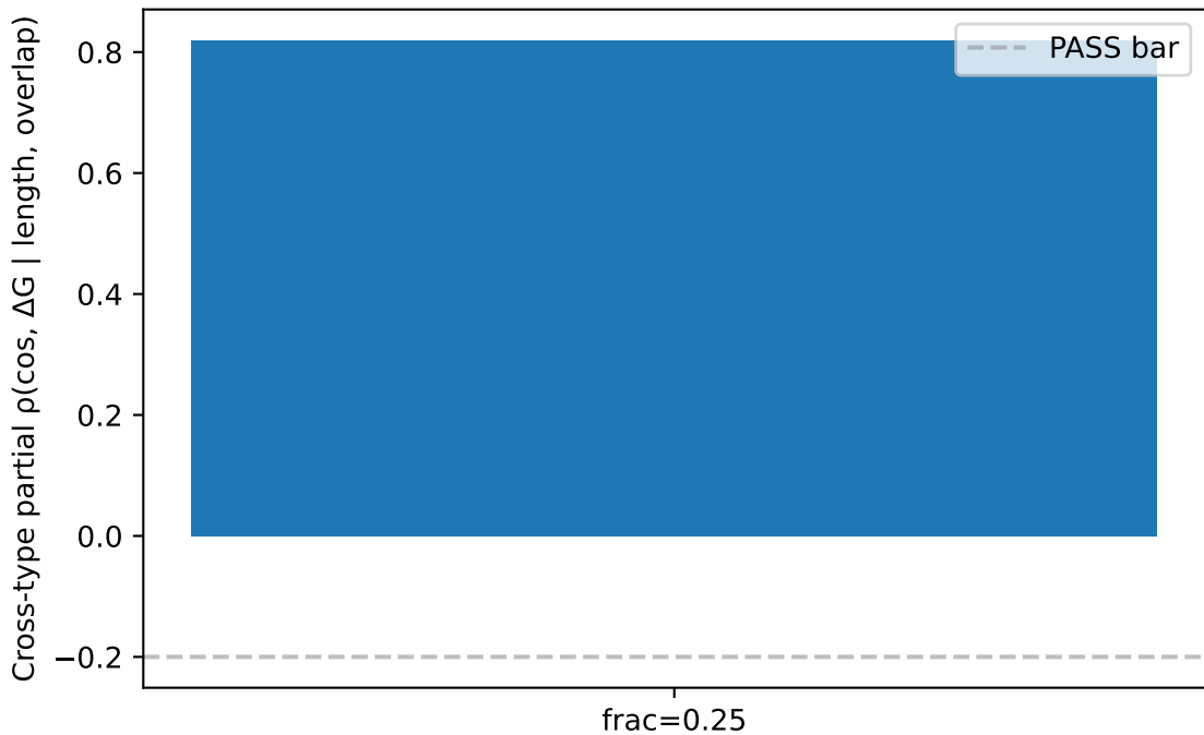
H4(a): cross-type cosine \rightarrow\Delta G controlling overlap
