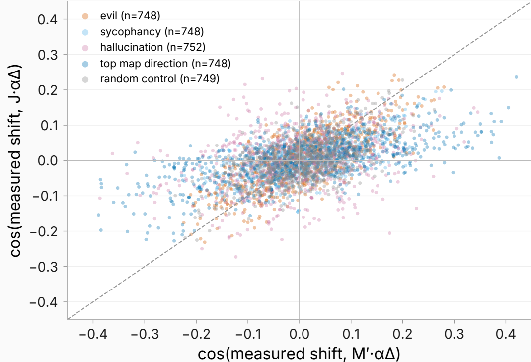
Steering prediction, per steered cell (prefill, unit-matched)
