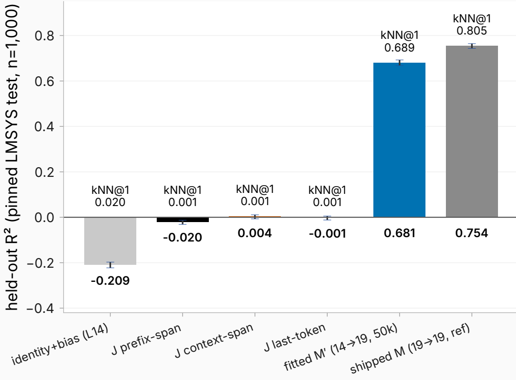
Answer-profile prediction: causal Jacobian vs fitted maps
