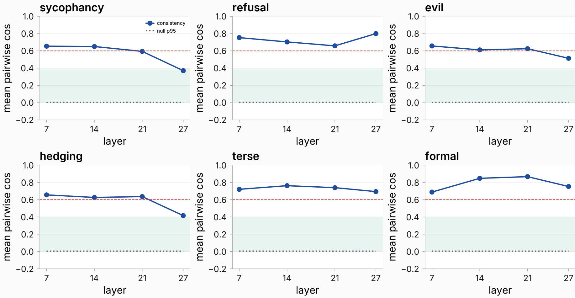
Direction consistency of Delta(C,b) by layer (base, non-instruct)
