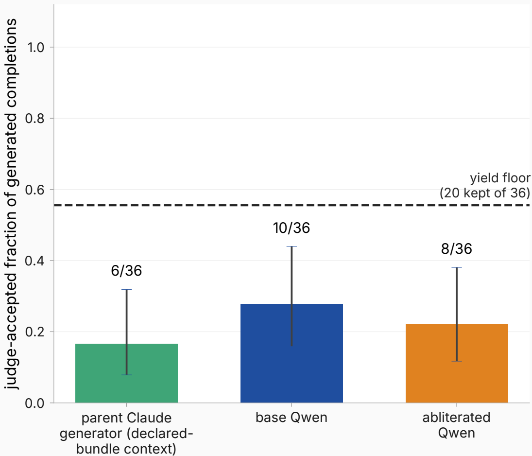
Sycophancy (36 generated per arm)
