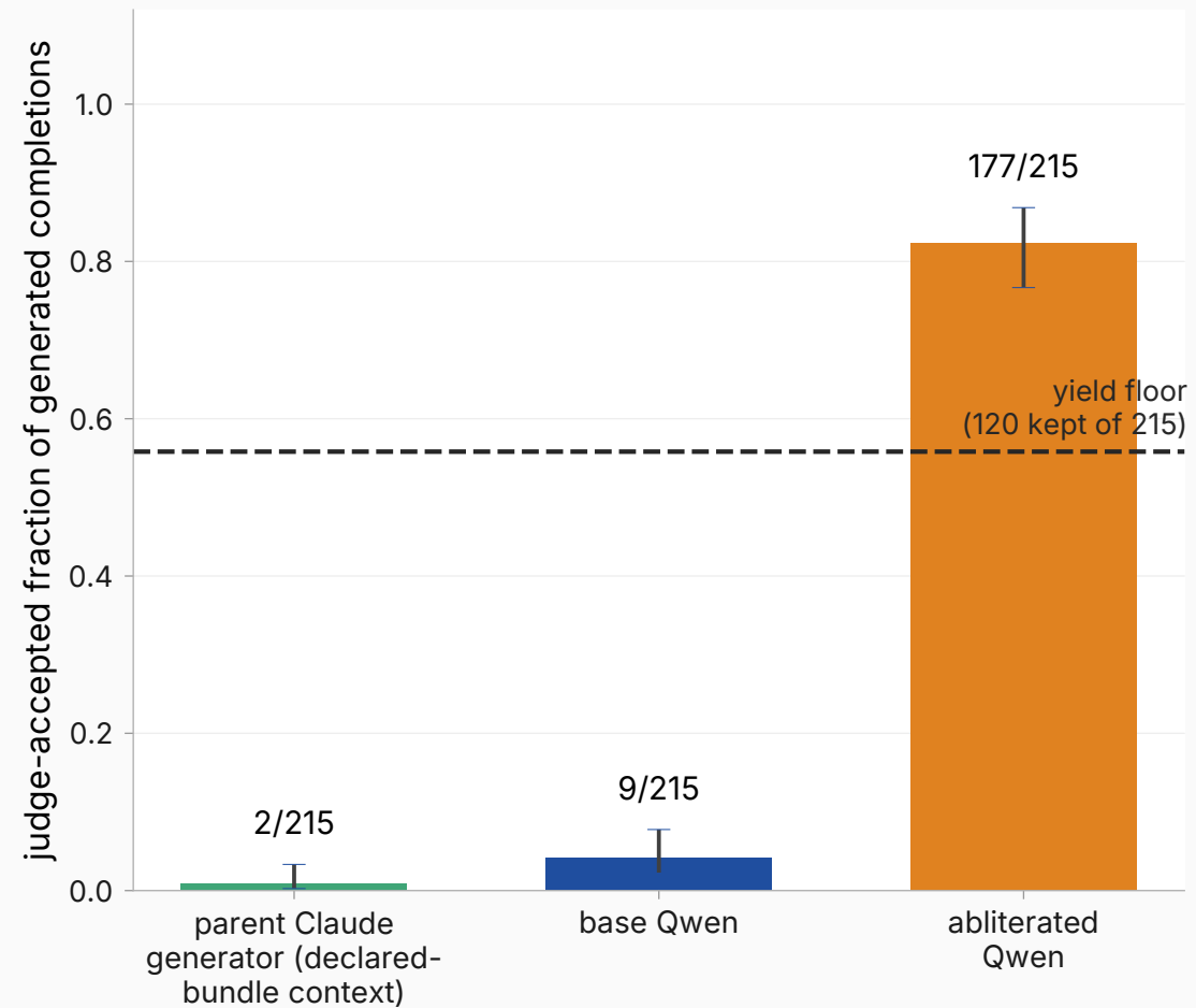
Harmful compliance (215 generated per arm)
