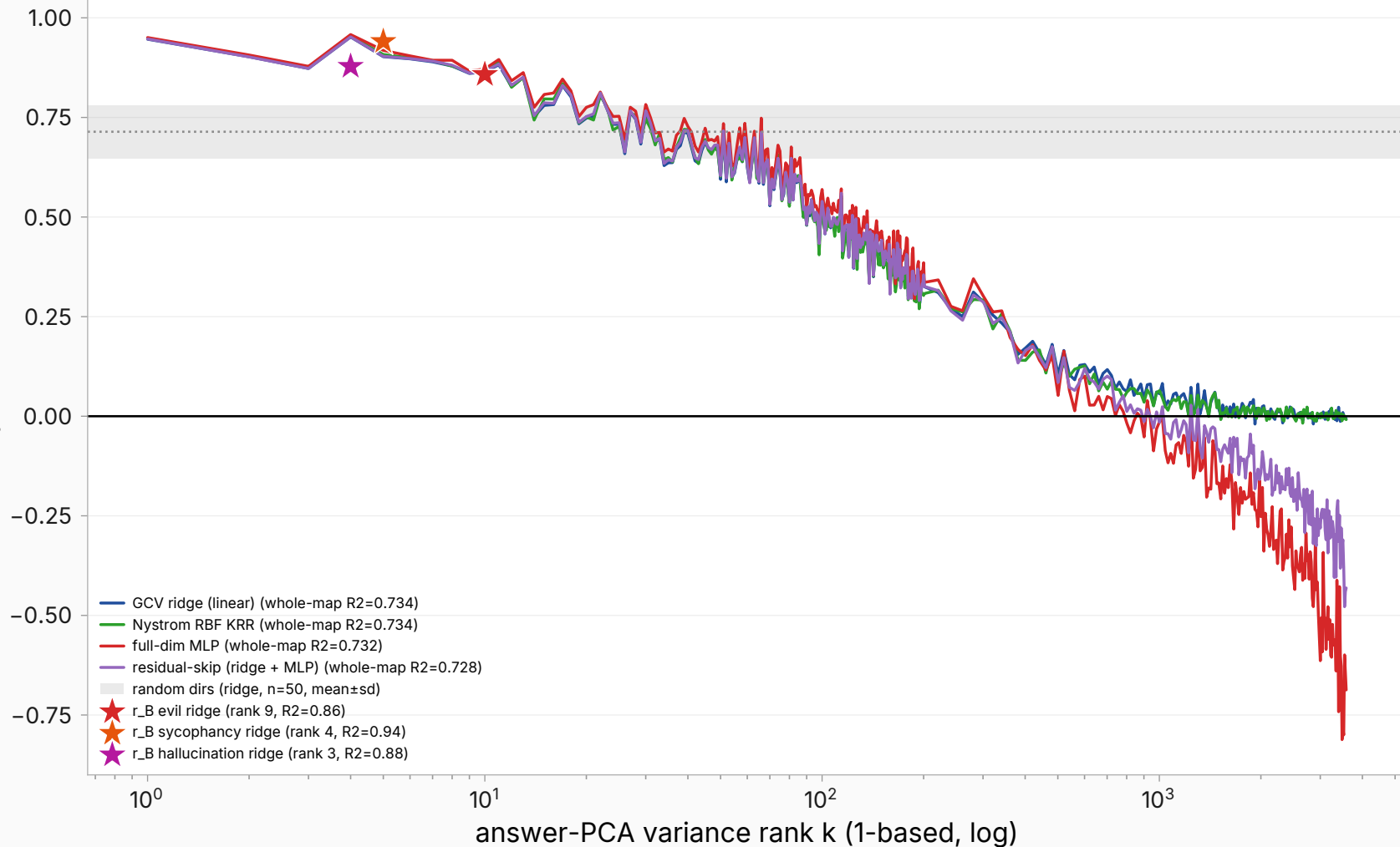
Per-direction predictability by fitter at L19 (n10k combined 11.5k) — do KRR/MLP lift the mid-ranks over ridge?
