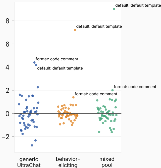
emergent misalignment
