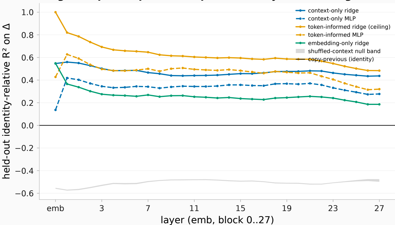
Single-step next-position \Delta predictability (answer segment, raw)
