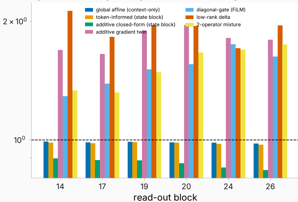
Spectral radius per map (dashed: instability threshold 1)
