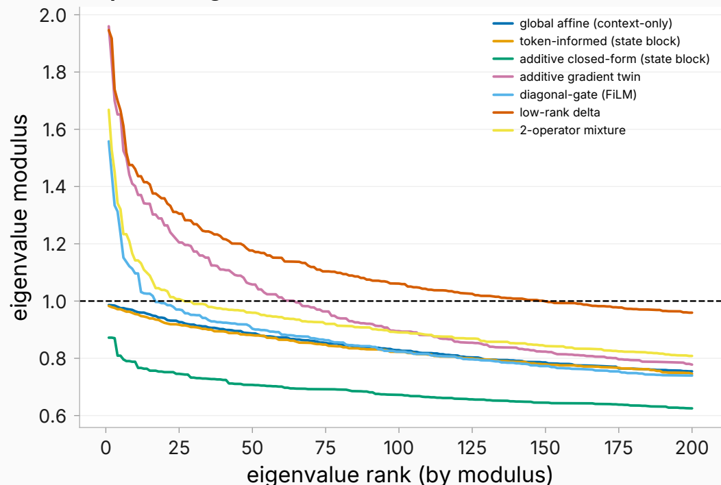
Top-200 eigenvalue moduli at block 20
