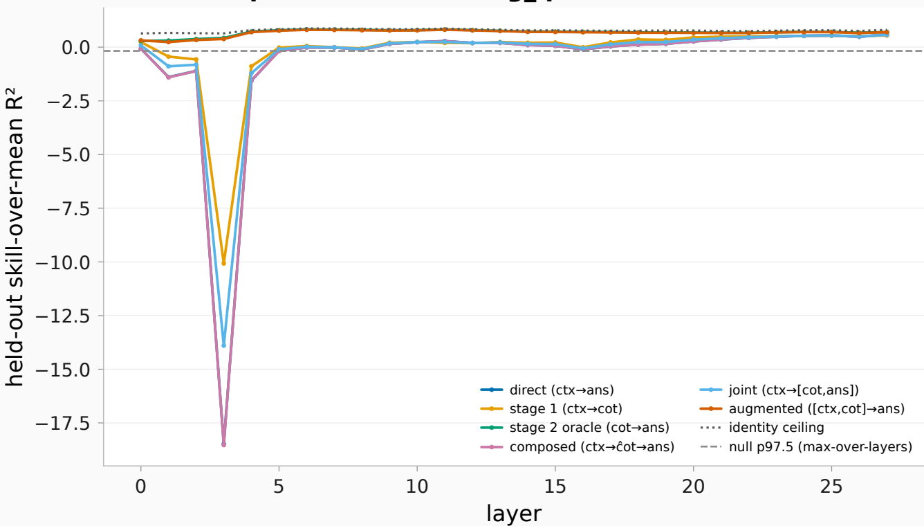
CoT-decomposition arms — avg_q, mean/mean, LOCO
