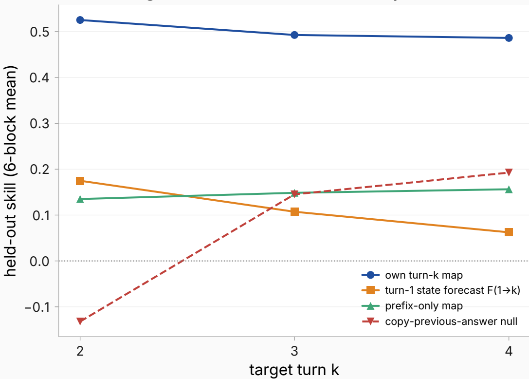
Forecasting answer k from earlier-turn inputs
