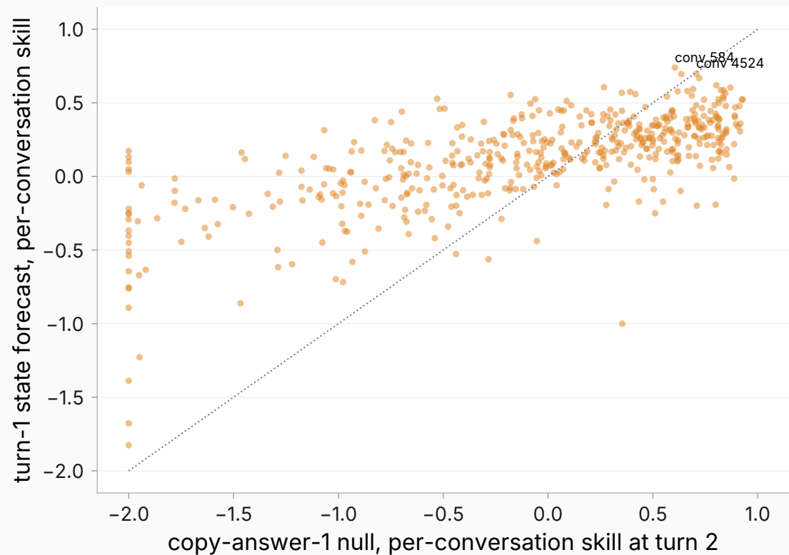
Per-conversation forecast vs null at turn 2 (clipped at -2)
