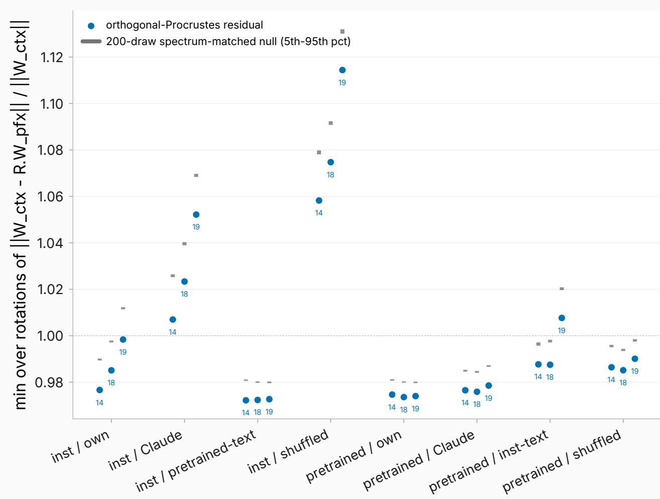
No rotation maps the prefix-arm operator onto the context-arm operator
