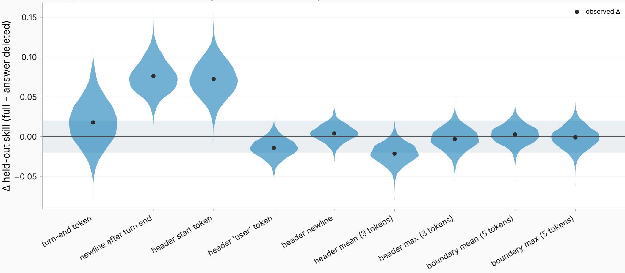
The 2,000 shared-index bootstrap draws behind each paired estimate
