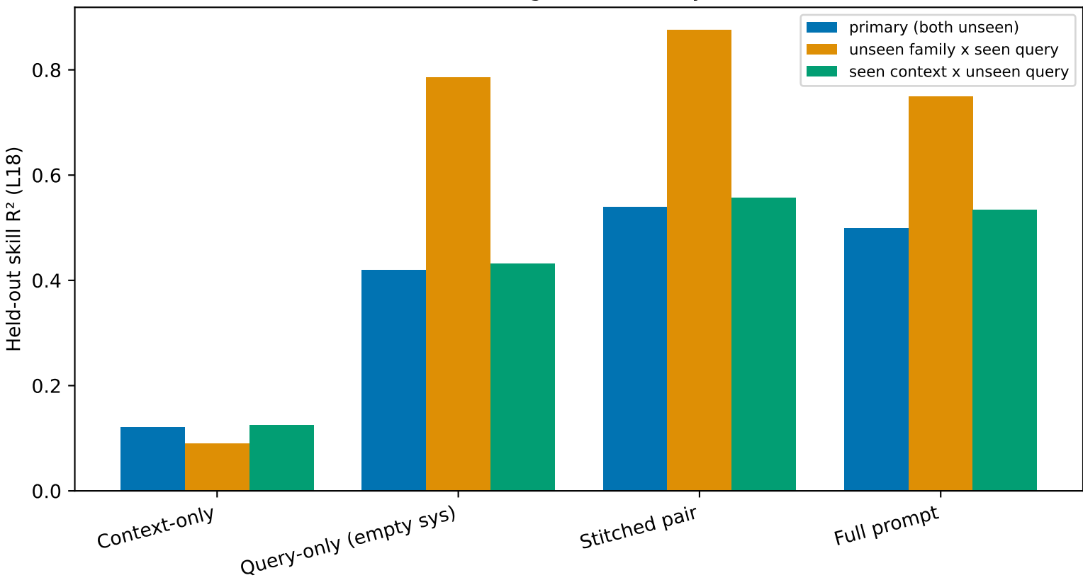
Fold regimes — betley
