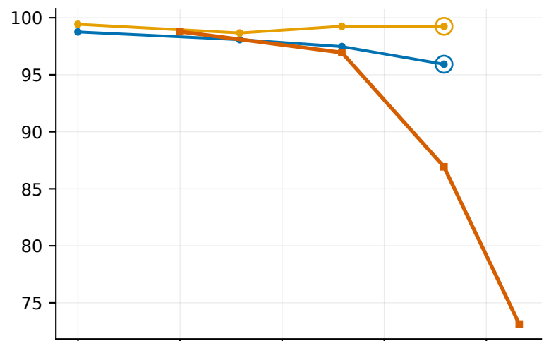
Hallucination II
