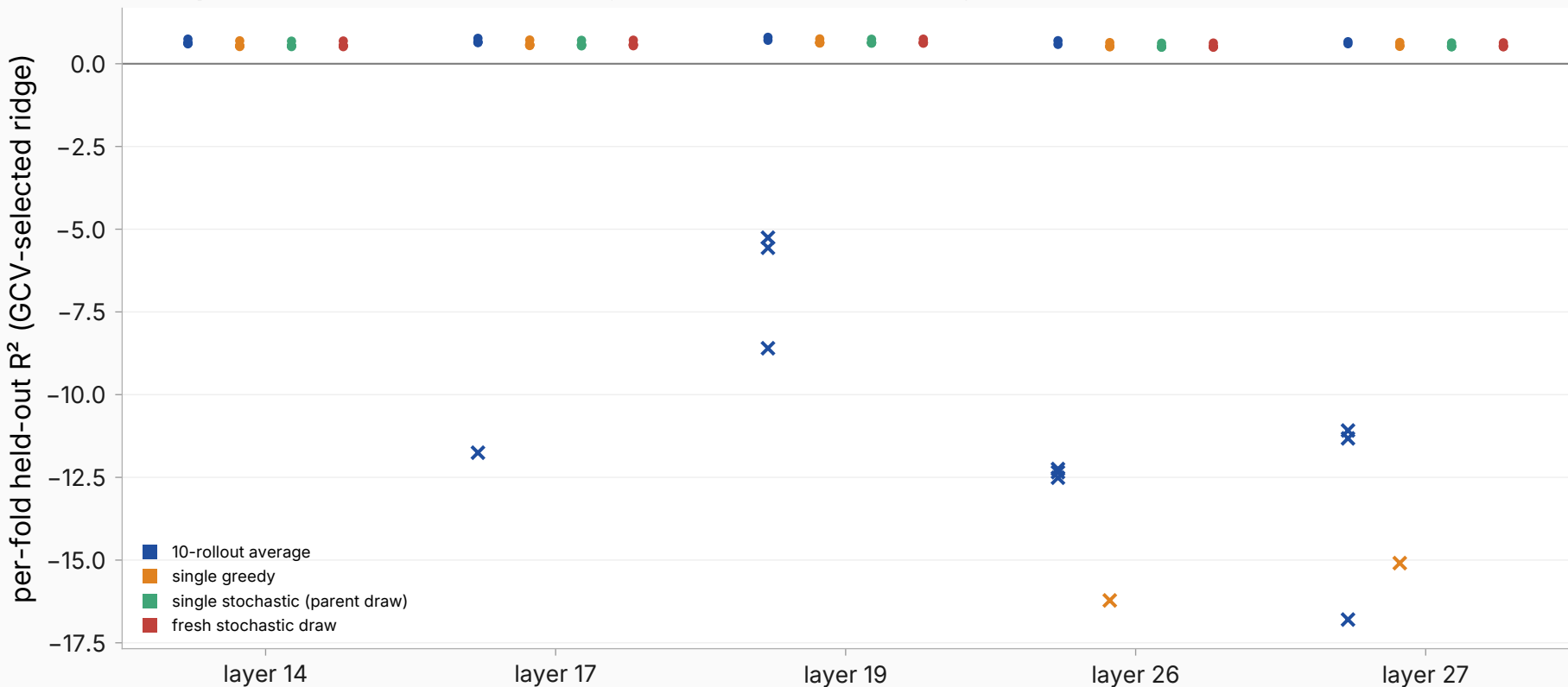
GCV per-fold fits: circles = healthy \lambda ( \geq 316 ), crosses = degenerate \lambda ( \leq 0.03 )
