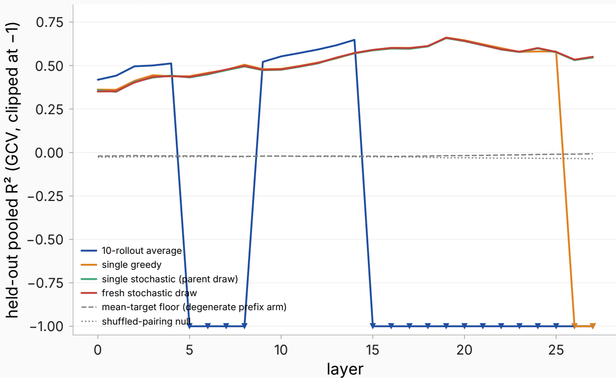
GCV map quality across layers (▼ = below -1 , degenerate \lambda )
