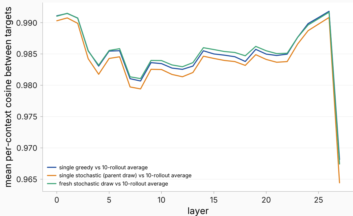
Answer-side target agreement across layers
