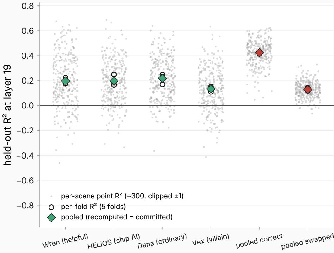
scene-aggregated — Qwen2.5-7B (base)
