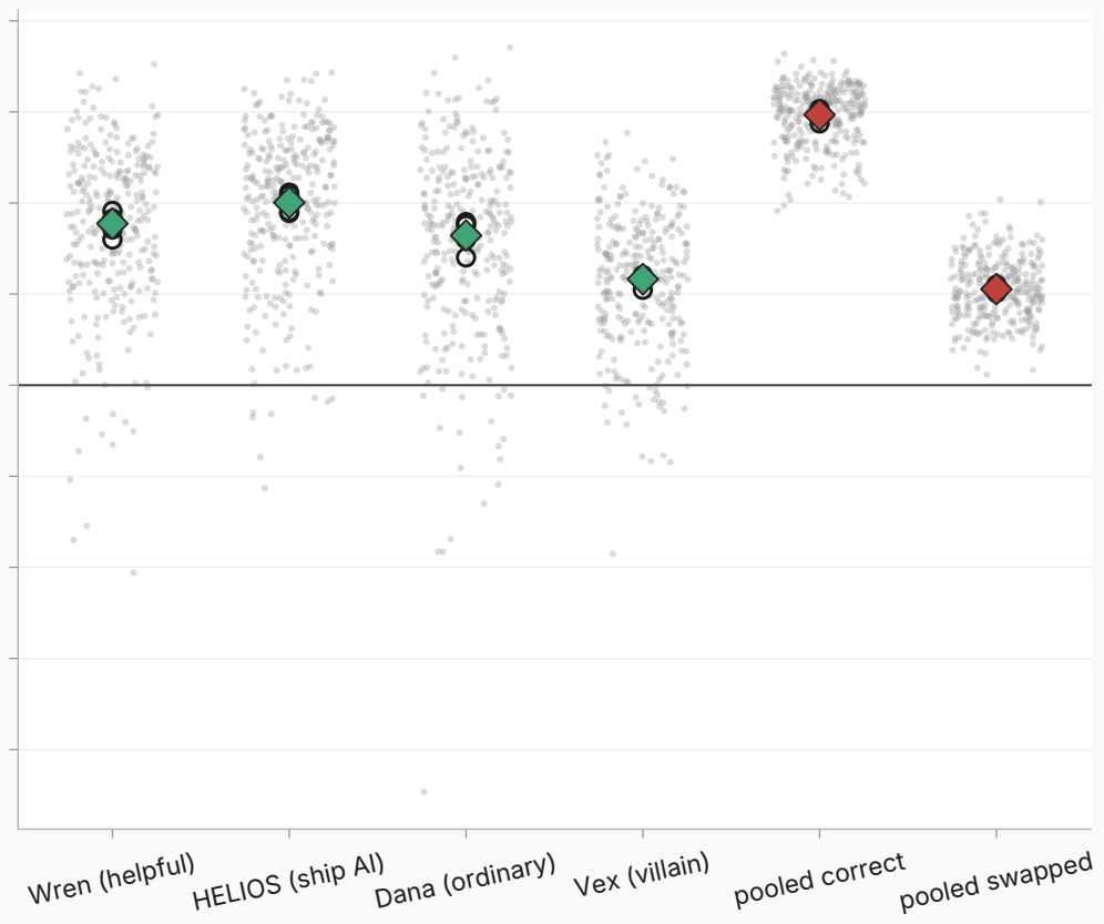
scene-aggregated — Qwen2.5-7B-Instruct
