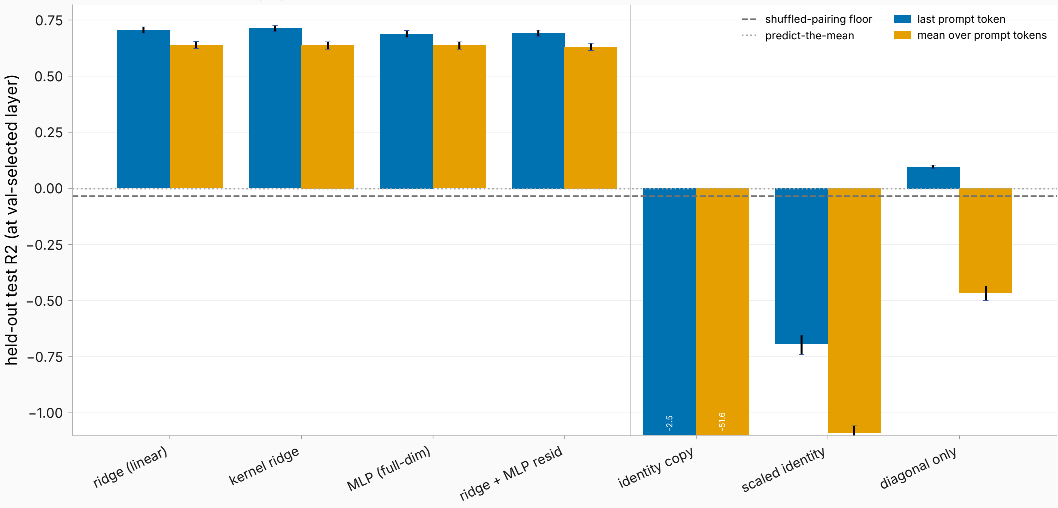
Context -> answer map: predictors vs baselines
