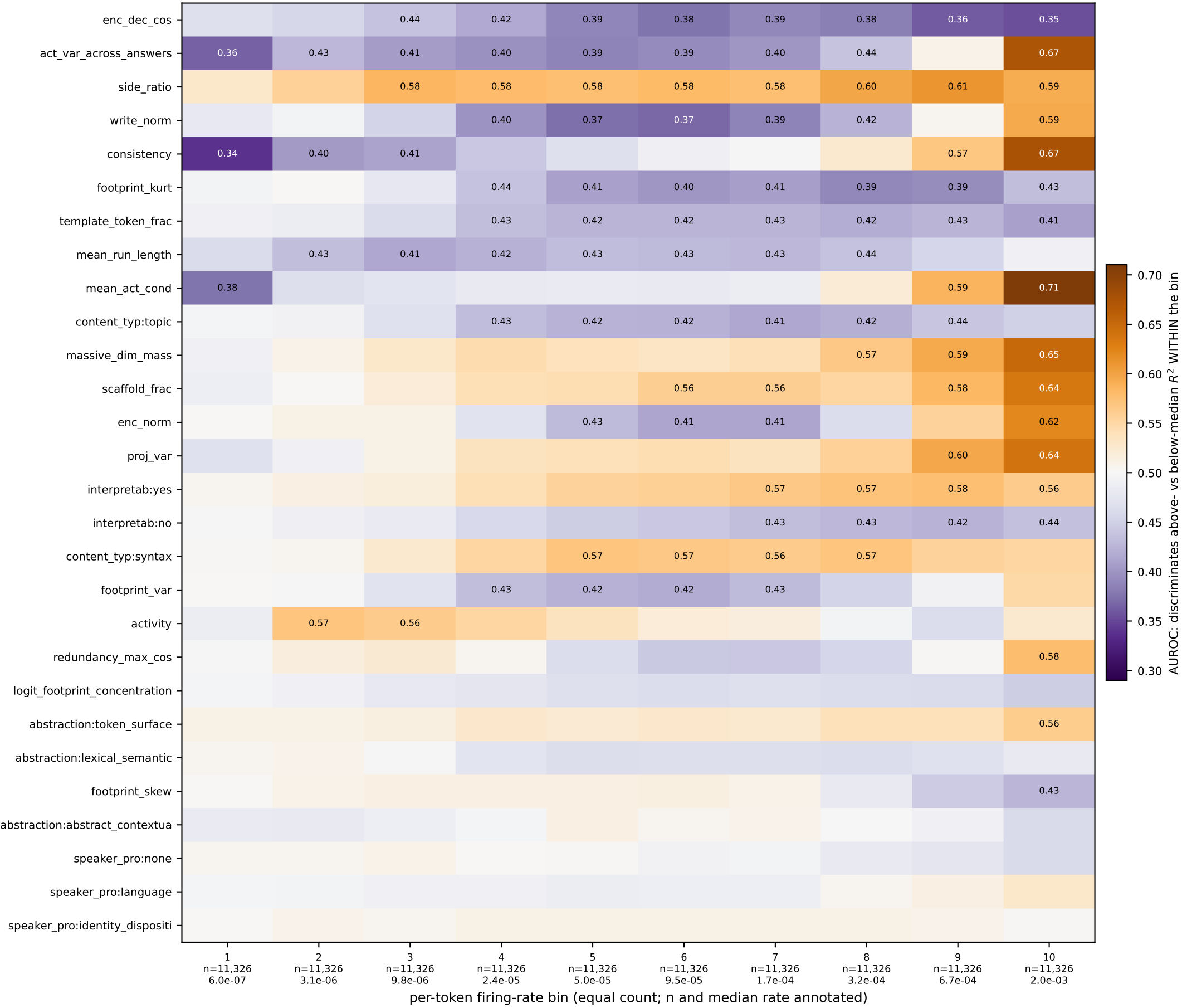
Which predictors work at matched firing rate? AUROC within per-token firing-rate bins — 0.5 = no discrimination; sorted by mean |AUROC - 0.5|
