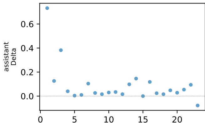
cosine layer-20 (baseline)
