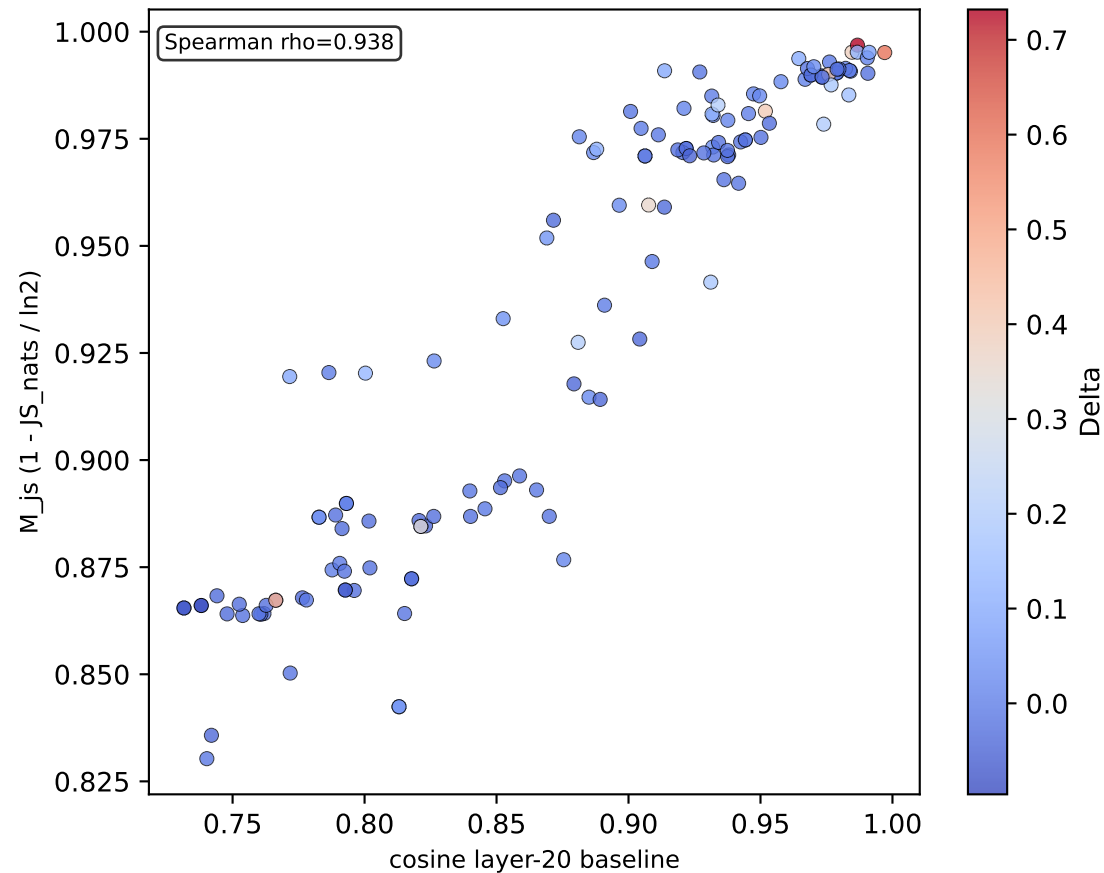
Predictor agreement (138 cells), color = Delta
