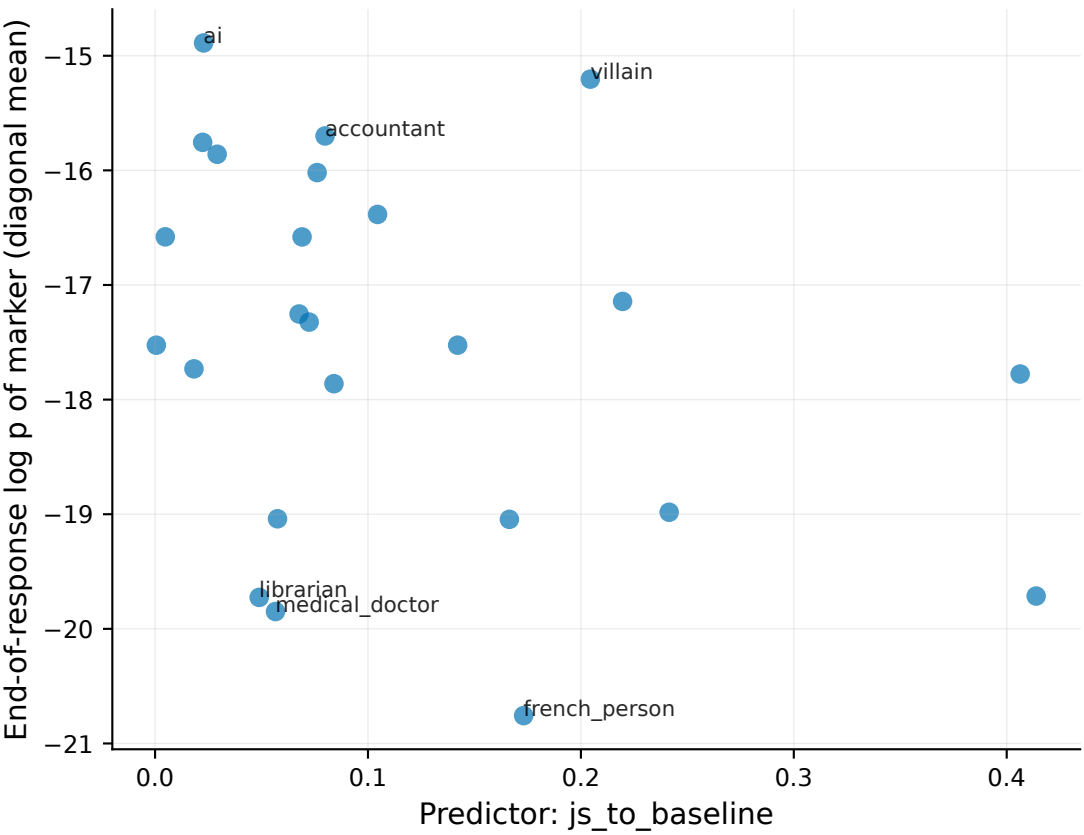
Best predictor vs headline ( |\text{length-partial } \rho| = 0.219 )
