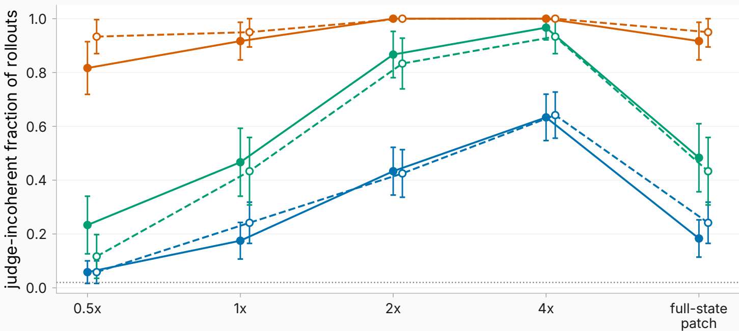
generation coherence per span and dose, steered vs shuffled-donor null (dotted line: 2.0 percent unpatched anchor baseline)
