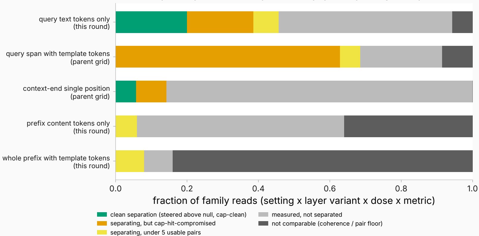
verdict composition per intervention span: follow-up spans vs parent-grid comparables
