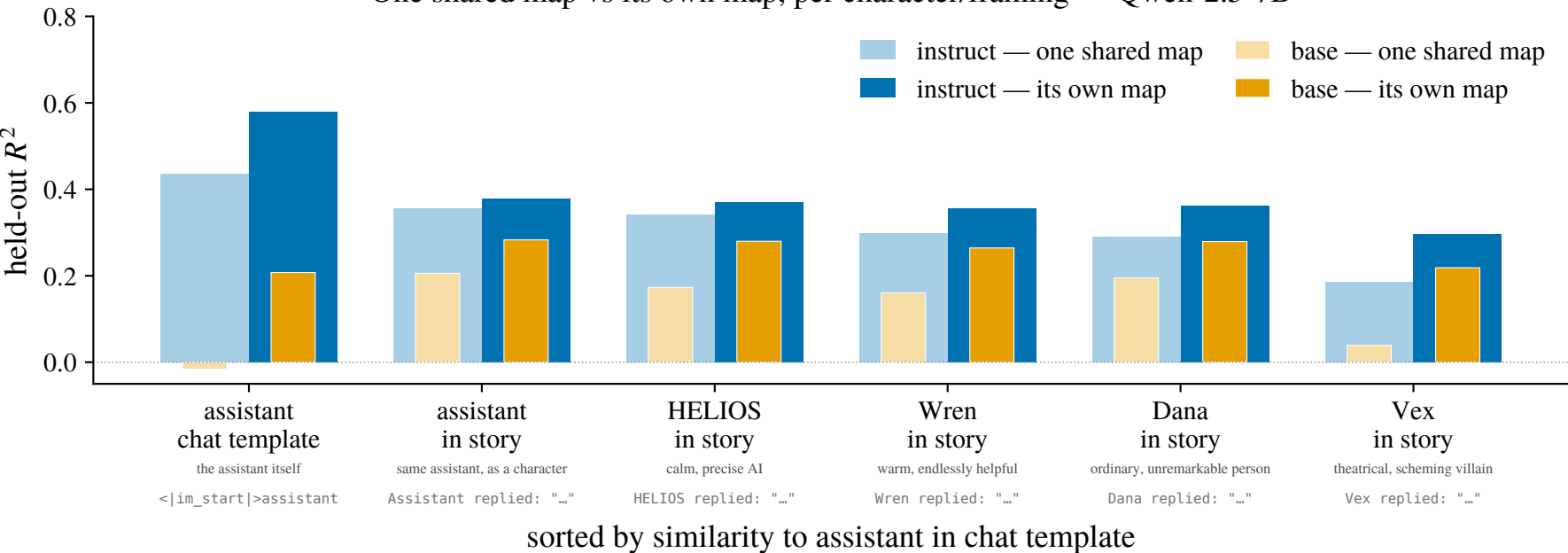
One shared map vs its own map, per character/framing — Qwen-2.5-7B
